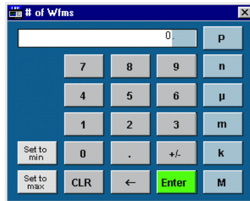
Figure 3-32: Virtual keypad
