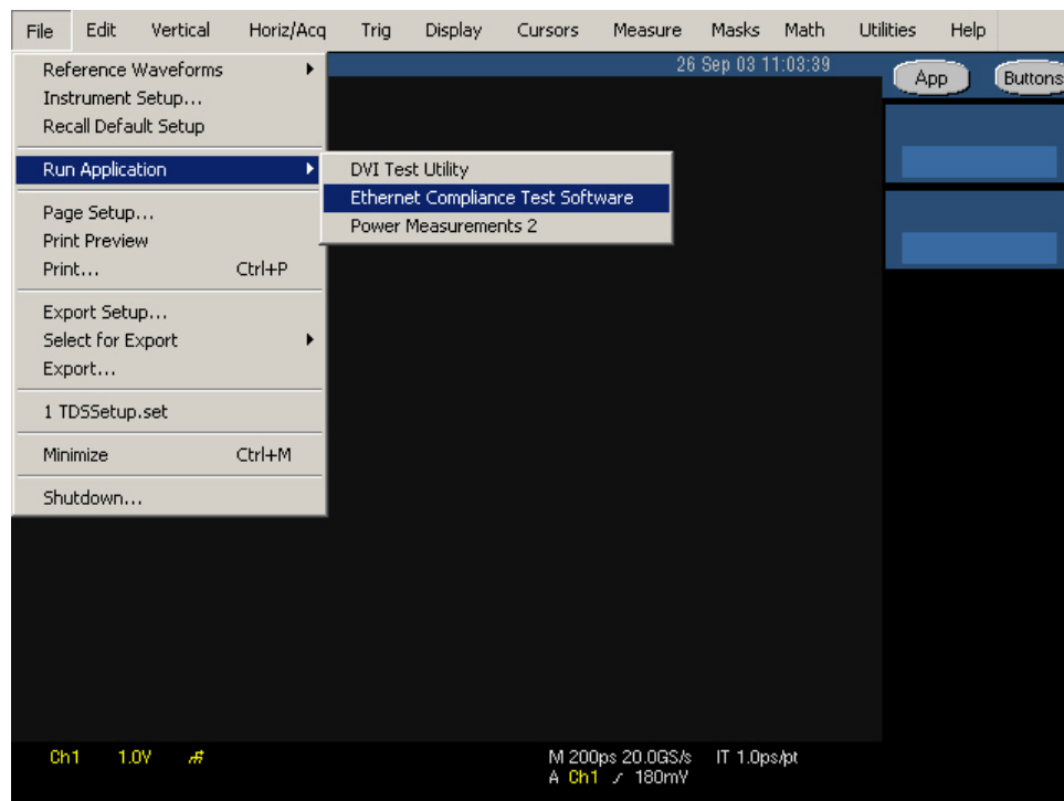
Figure 2-1: Run application
