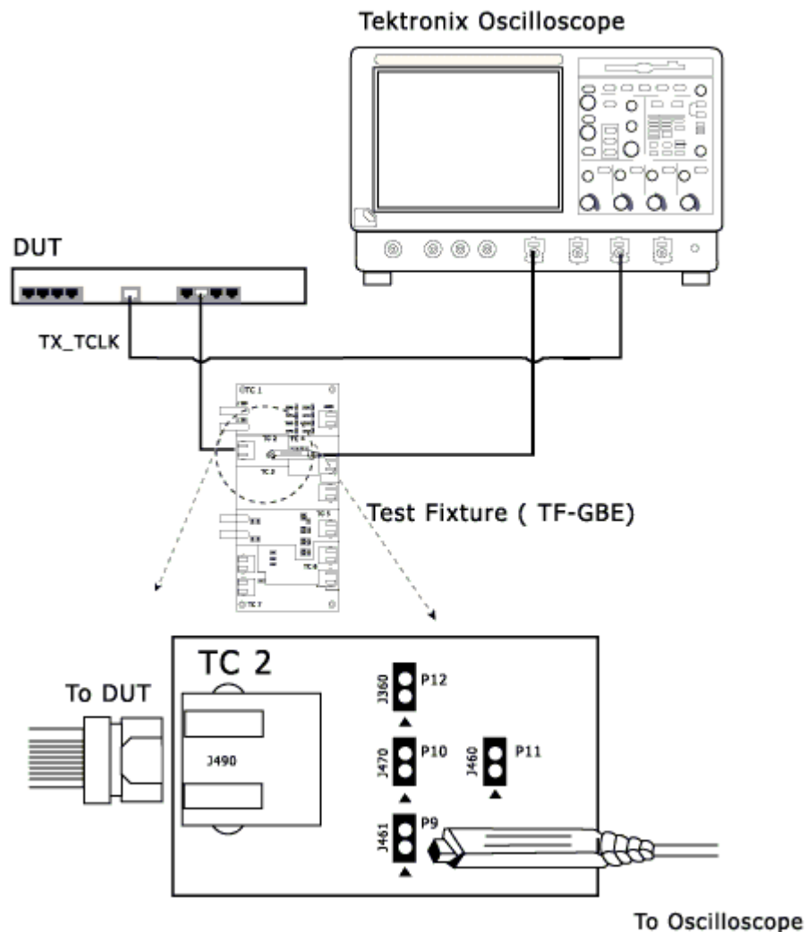
Figure 6-9: 1000BASE-T Step 2 Connections for Jitter Slave Filtered
