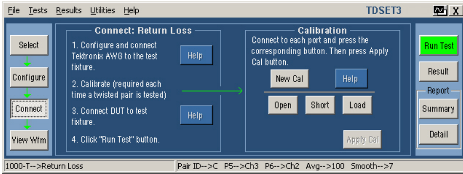
Figure 18-2: Connect pane of 1000BASE-T Return Loss
