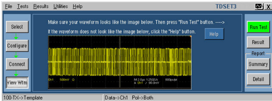
Figure 12-1: 100BASE-TX View Waveform for all tests except Return Loss
